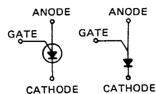
Fig. 9-9 Symbol of PUT
