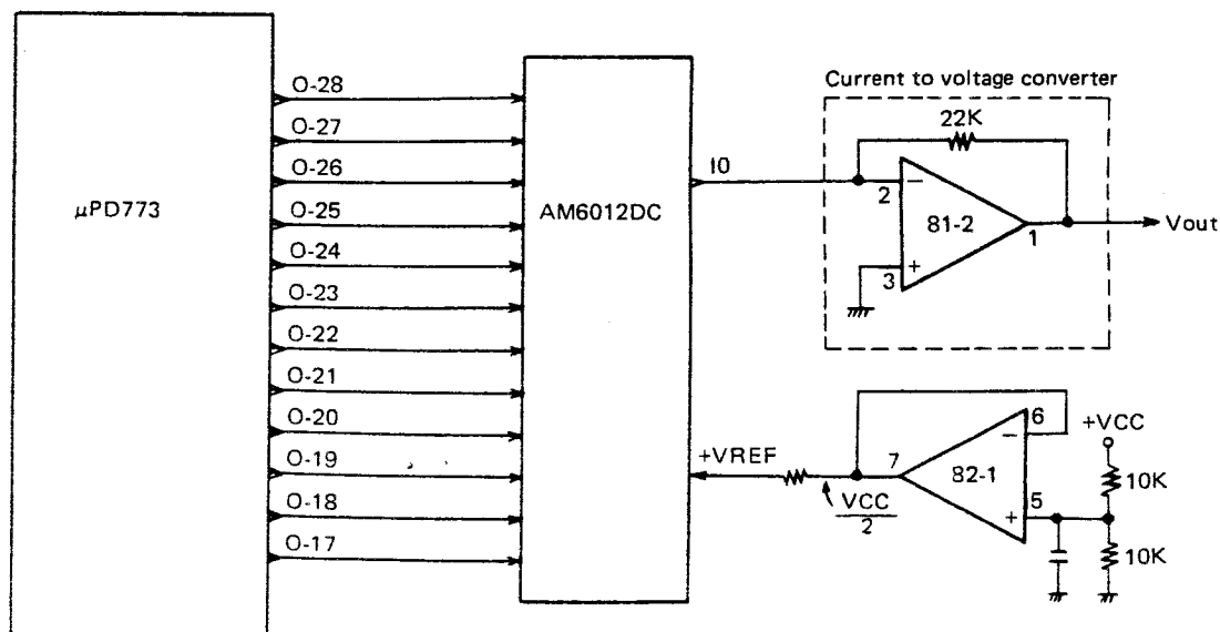
Fig. 6-3 D/A converter block
