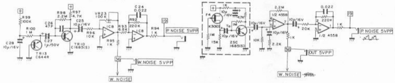
NOISE CIRCUIT NO.2 (SERIAL NO.132828 ~ )
